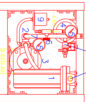
FRONT VIEW 21.25"
