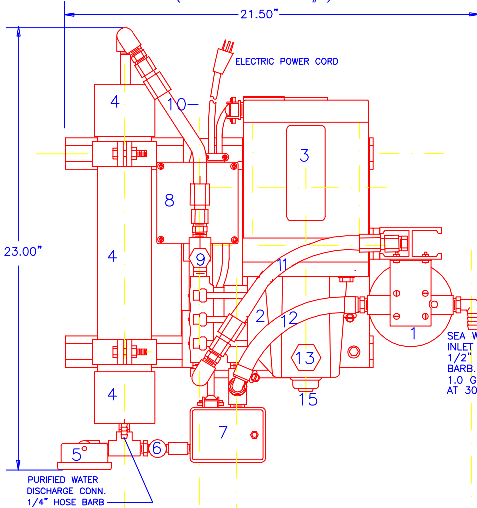
TOP VIEW 1"=5"
