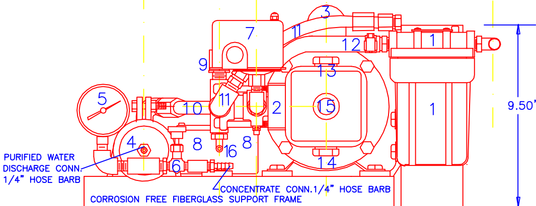
FRONT VIEW 1"=5"
